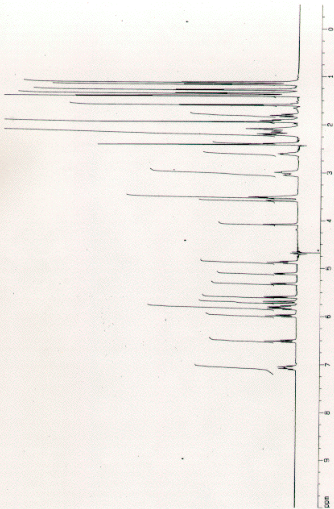
500 MHz ^1\text{H} NMR of (+)-Discodermolide in 50% \text{D}_2\text{O} in \text{CD}_3\text{CN} .
